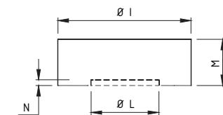
Plaque de charge (option) - Upper Plate (option)
